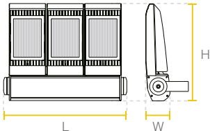
300W Sylveo LED - Extra large
